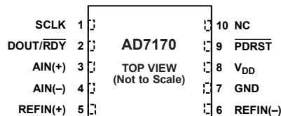
Figure 5. Pin Configuration
